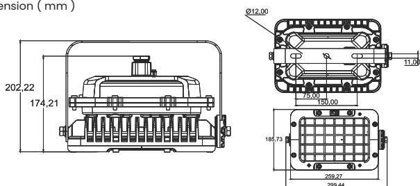
Dimension ( mm )
