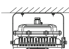
Ceiling Type
